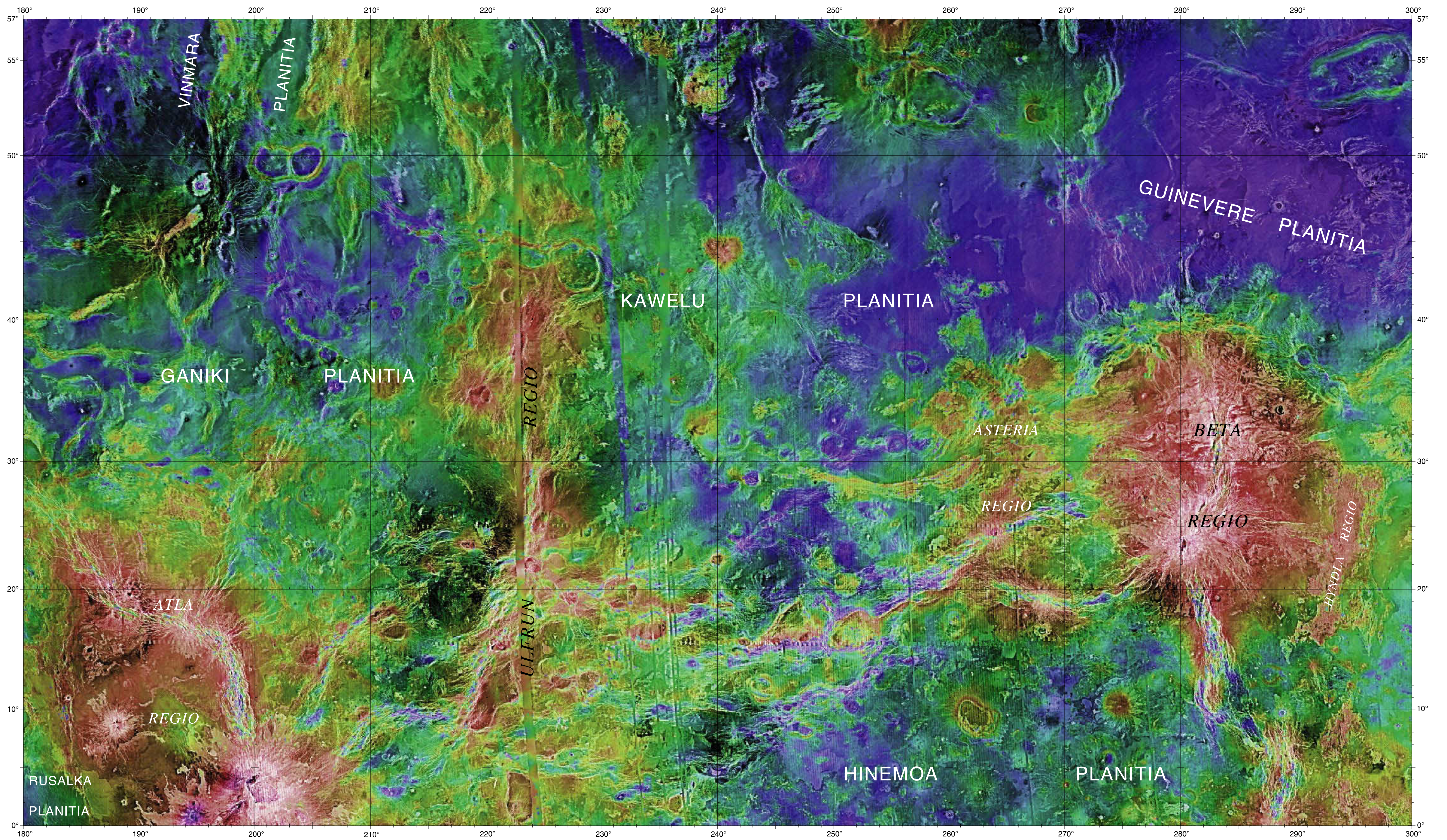
ALTIMETRIC RADAR IMAGE MAP OF THE GUINEVERE PLANITIA REGION OF VENUS
