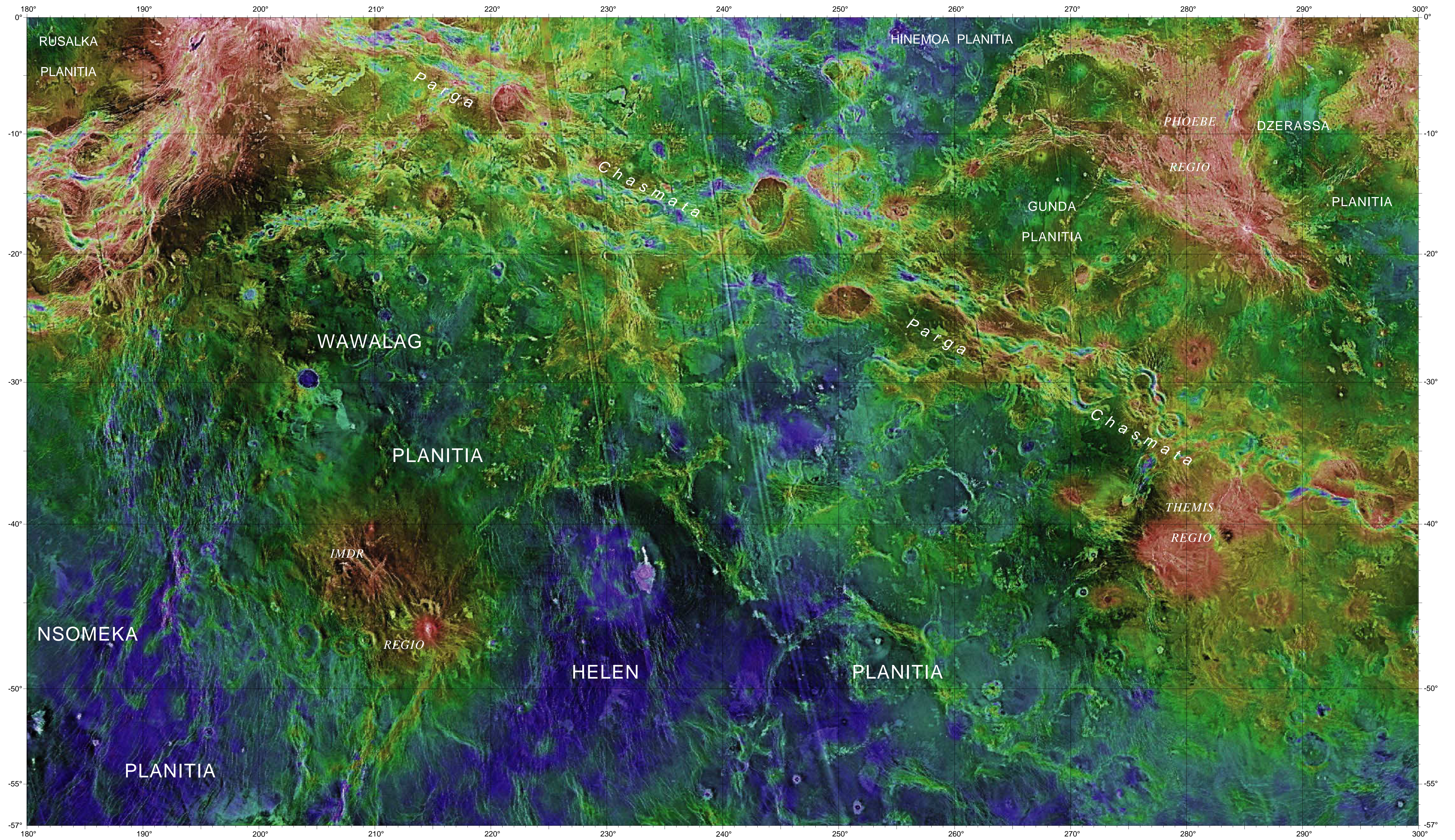
ALTIMETRIC RADAR IMAGE MAP OF THE HELEN PLANITIA REGION OF VENUS
