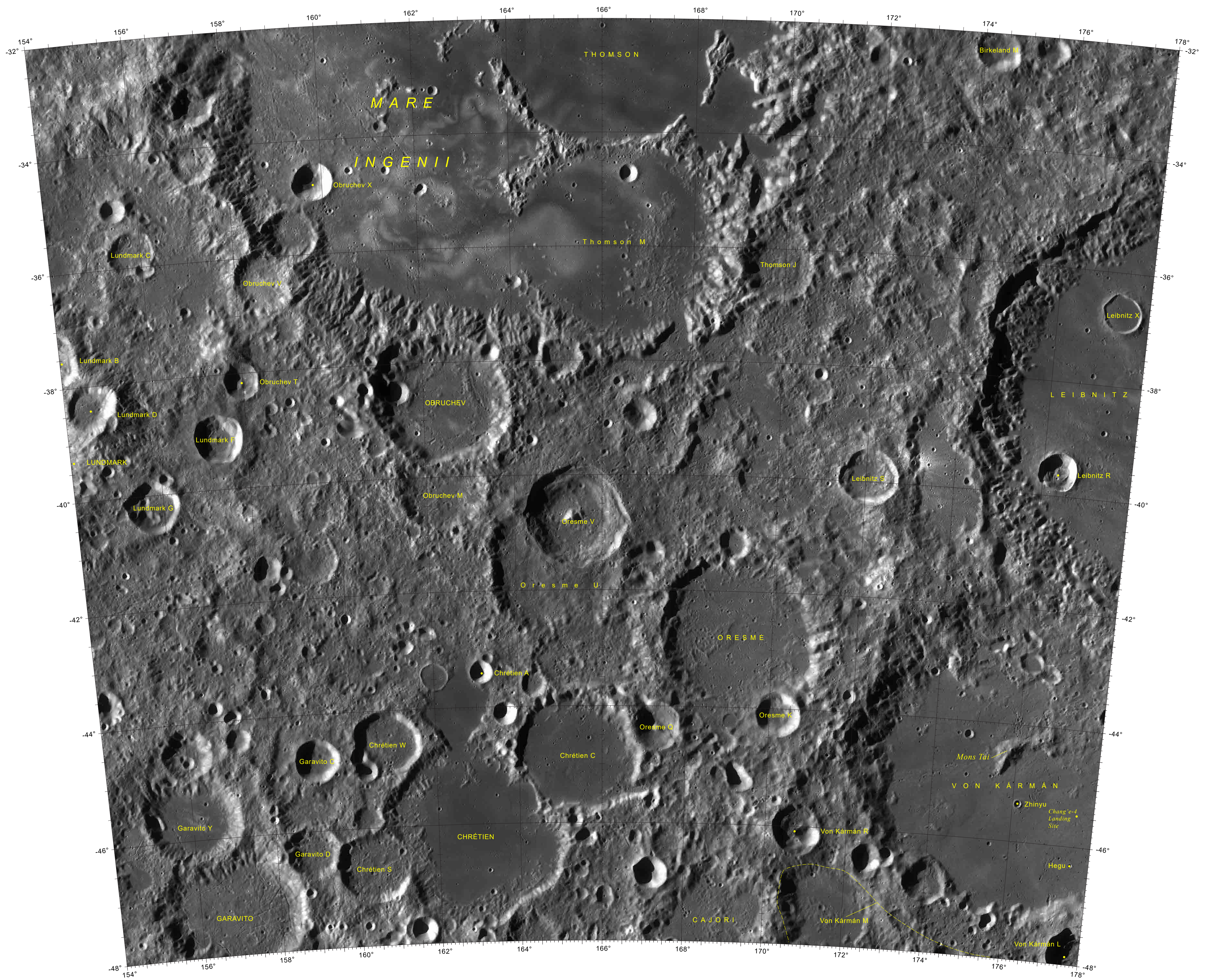
LAC 119 Scale 1:1,000,000 Lambert Conformal Projection
