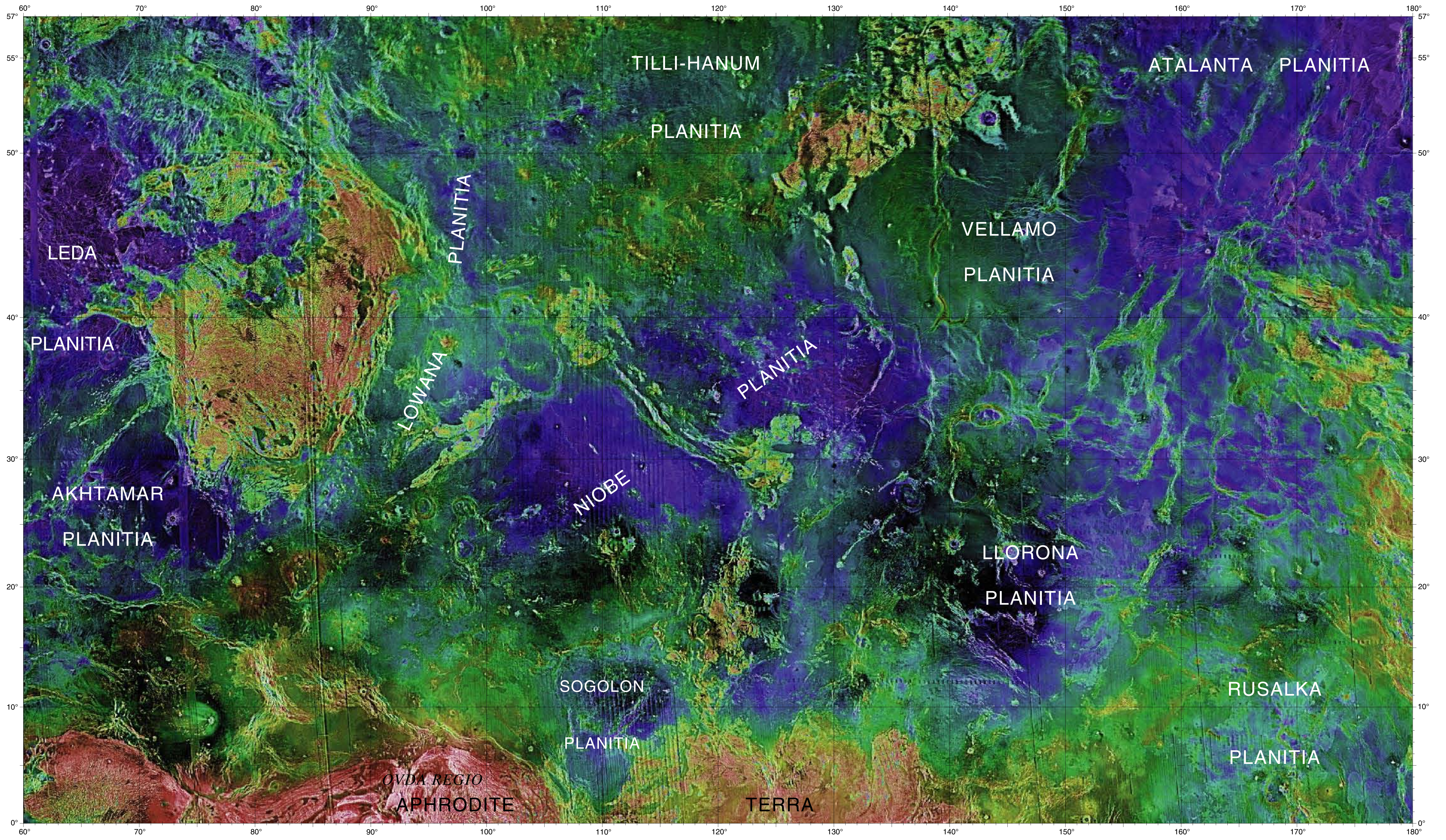
ALTIMETRIC RADAR IMAGE MAP OF THE NIOBE PLANITIA REGION OF VENUS
