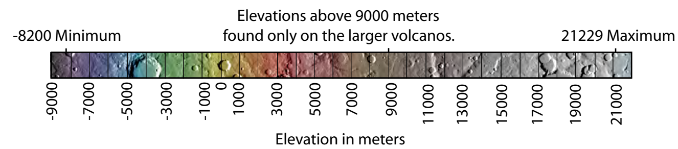
Phoenicis Lacus, MC-17 Mercator Projection
