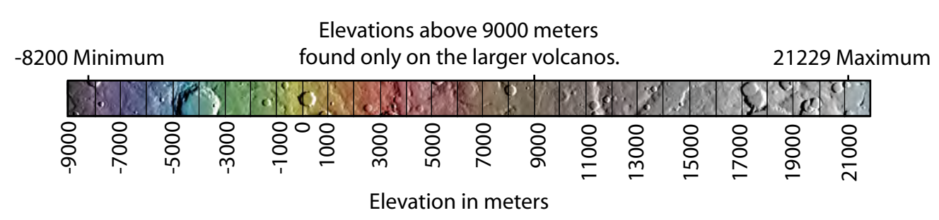
Cebrenia, MC-7 Lambert Conformal Conic Projection
