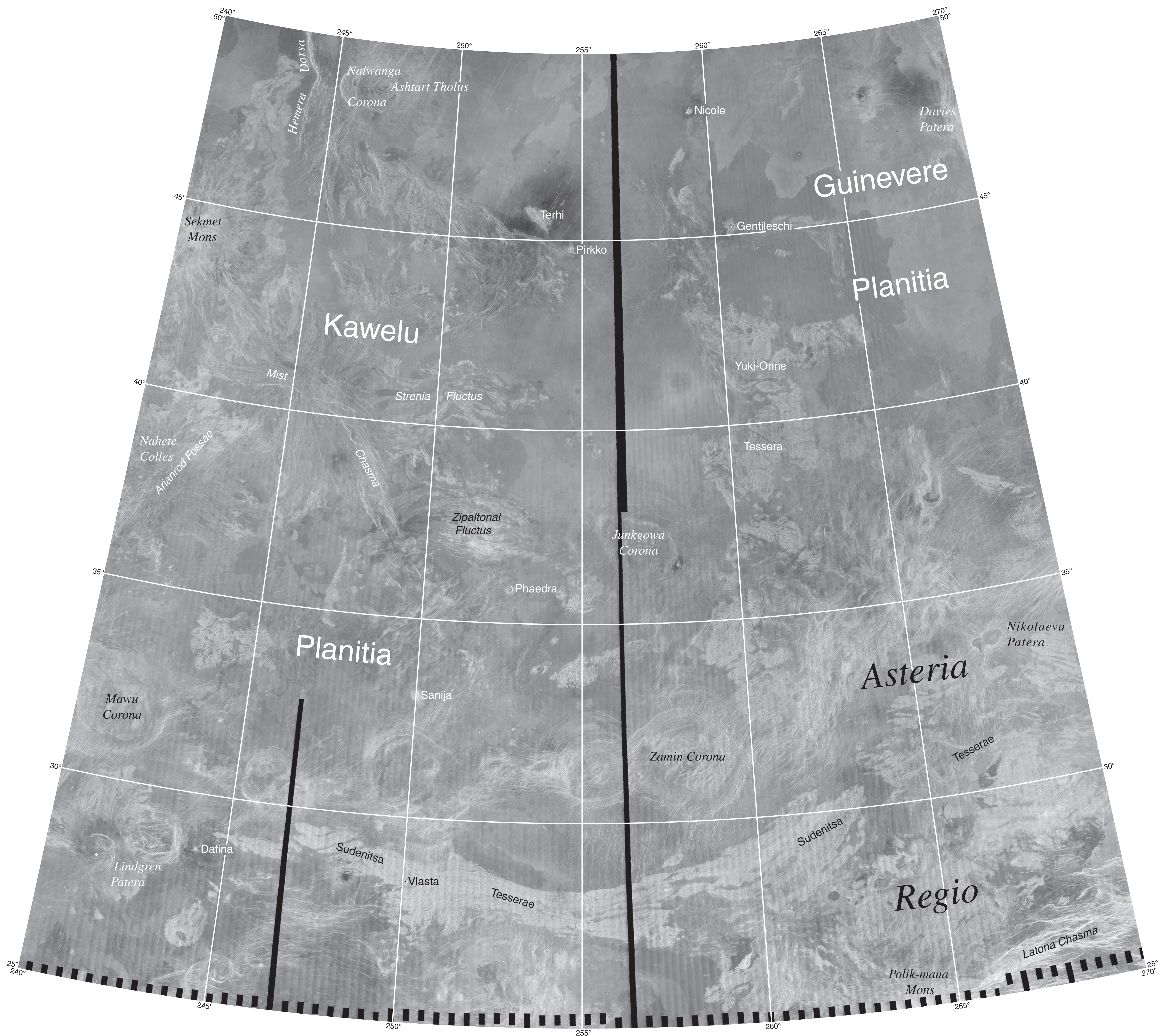
Kawelu Planitia, V-16 Lambert projection
