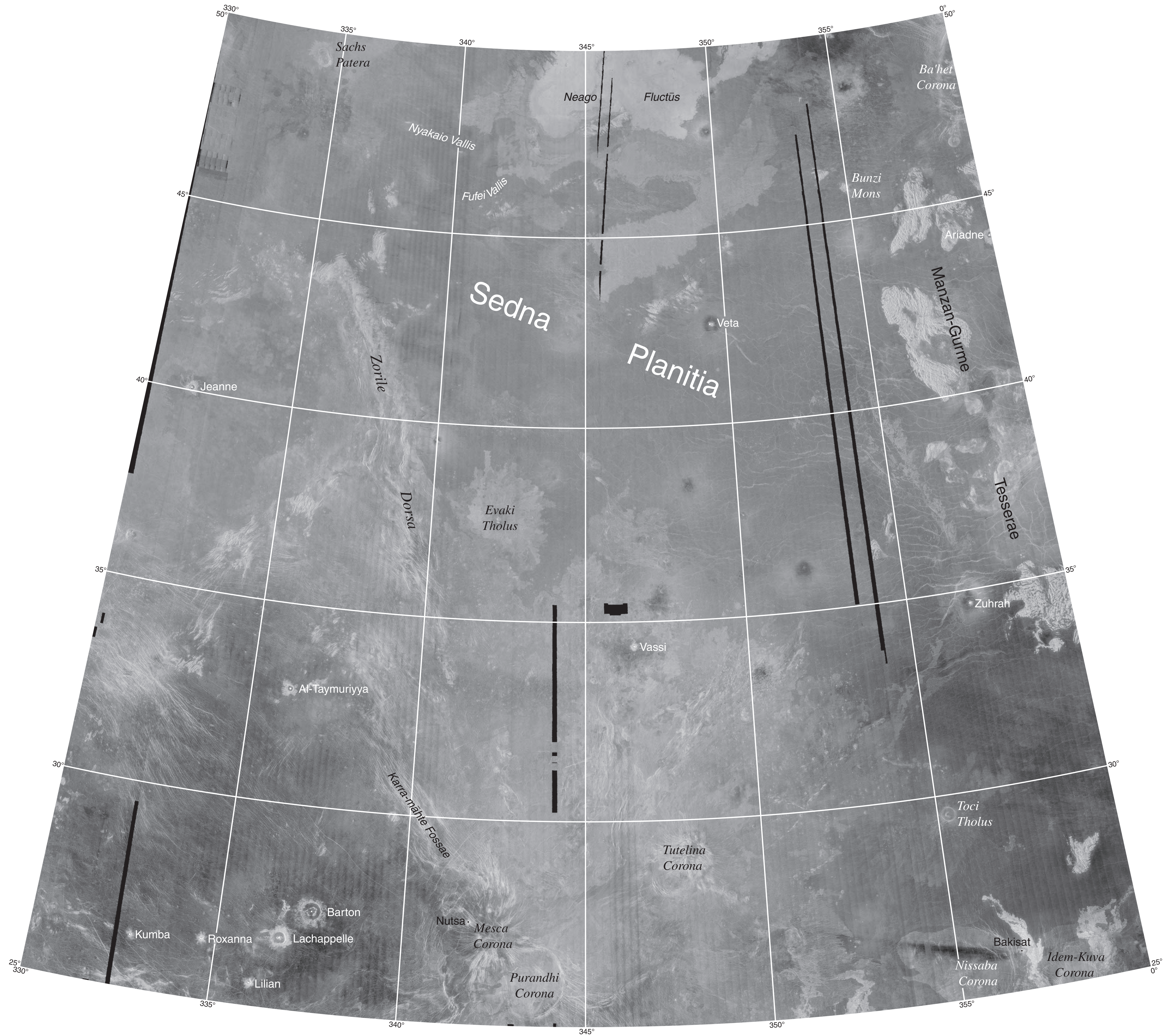
Sedna Planitia, V-19 Lambert projection
