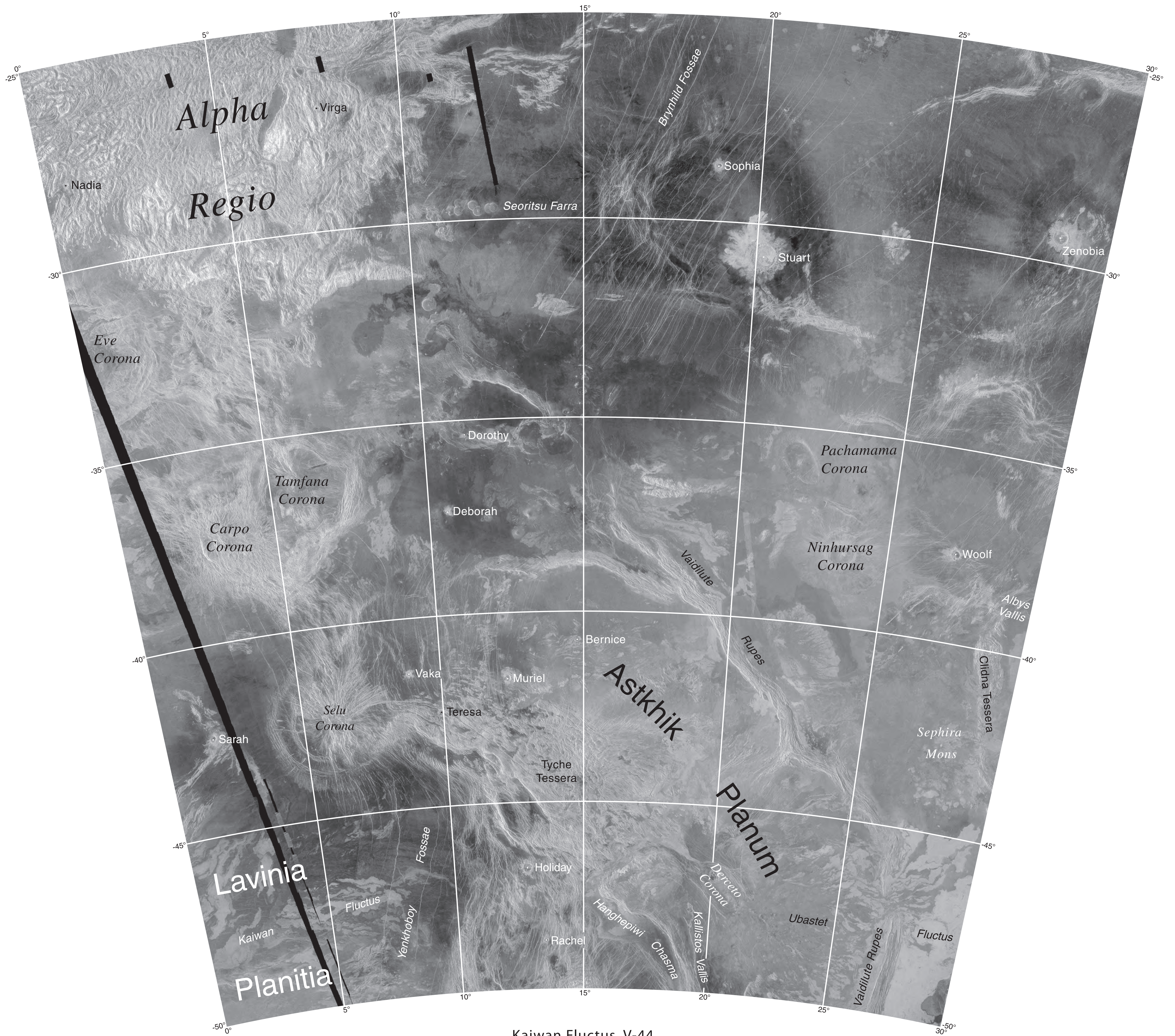
Kaiwan Fluctus, V-44 Lambert projection
