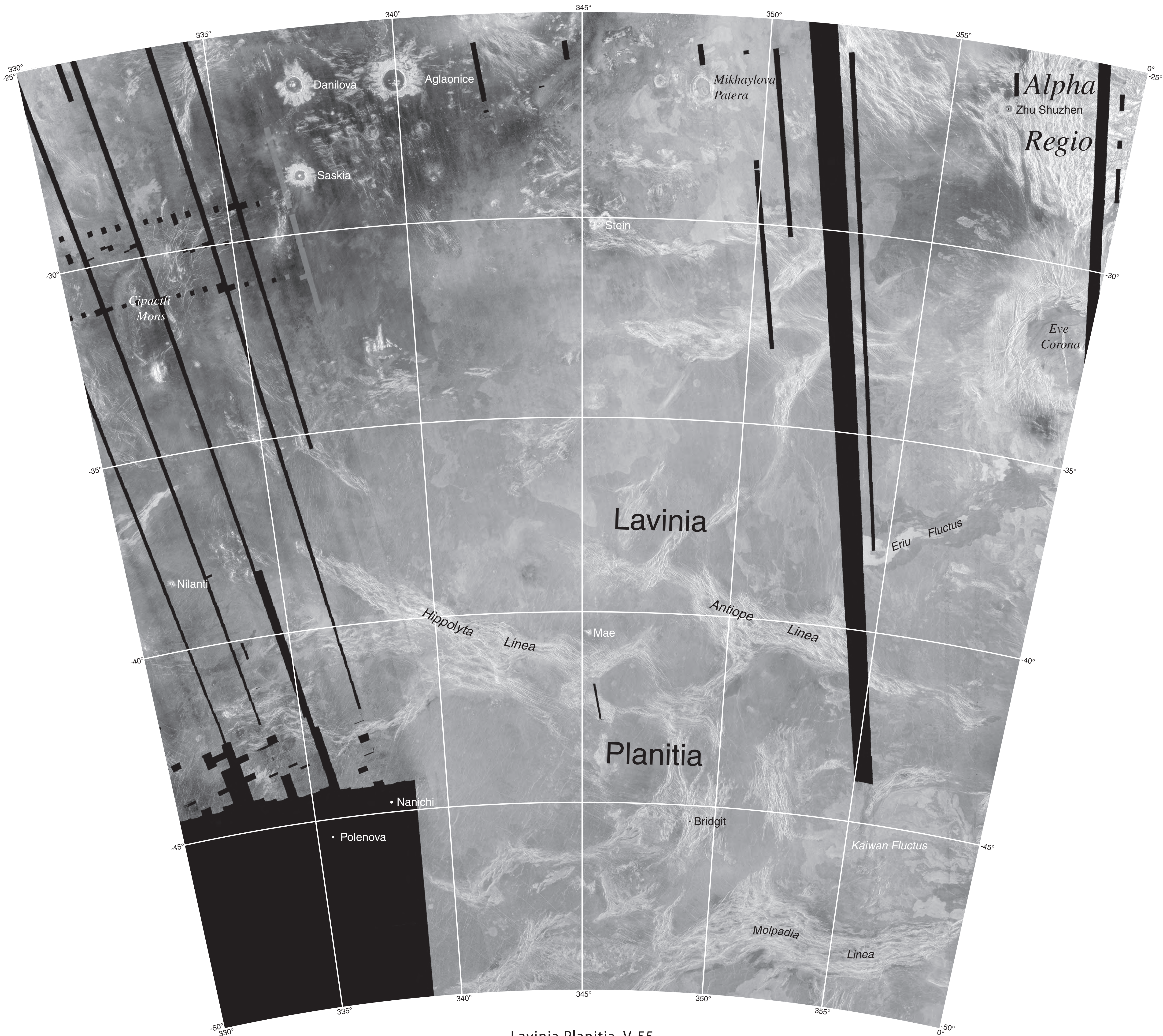
Lavinia Planitia, V-55 Lambert projection
